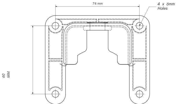
WALL BRACKET DRILL PATTERN
